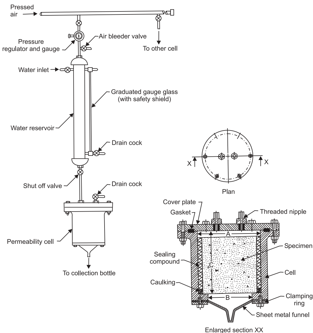
Fig. 12.5 Permeability Test Set-Up (Schematic)
