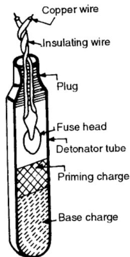
Fig. 3.5 Electrical Detonator
