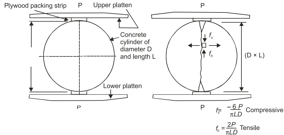
Fig. 10.17 Loading Arrangement of Split Tensile Strength Test
