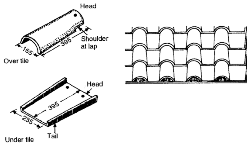
Fig. 2.16 (e) Spanish Tiling
