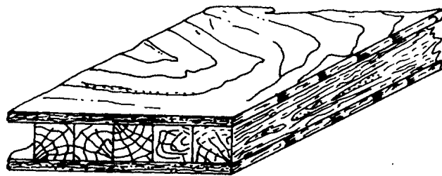
Fig. 4.26 Block Board
