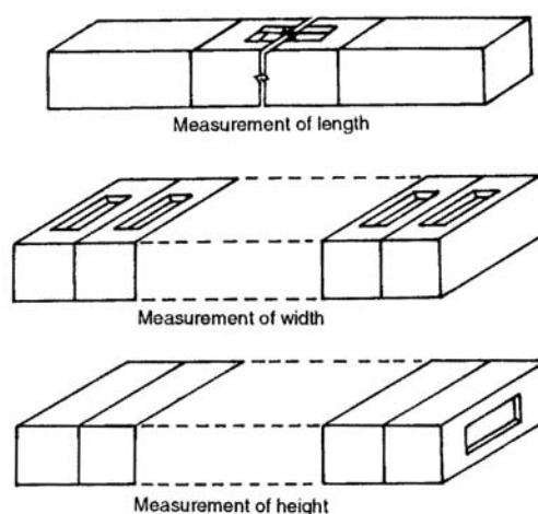
Fig. 2.14 Measurement of Tolerances of Common Building Bricks
