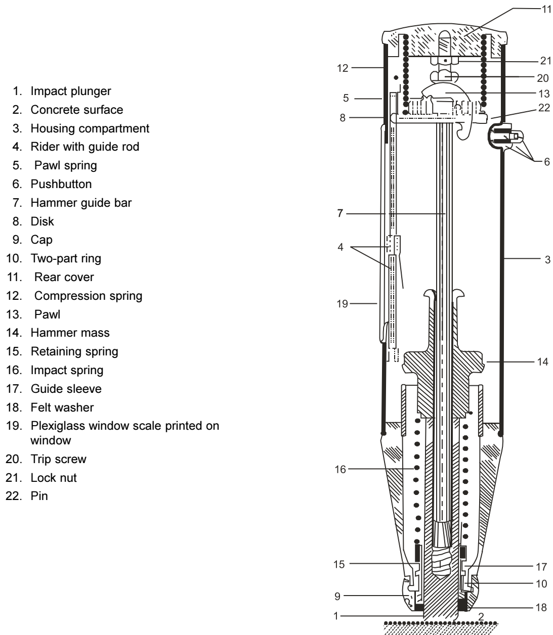
Fig. 10.38 Concrete Test Hammer
