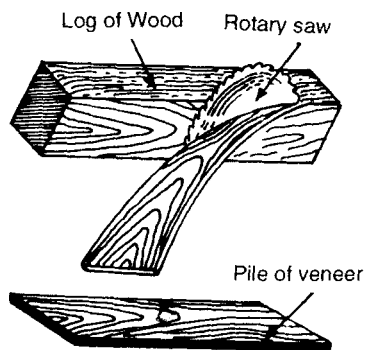
Fia. 4.24 Sliced Veneer
