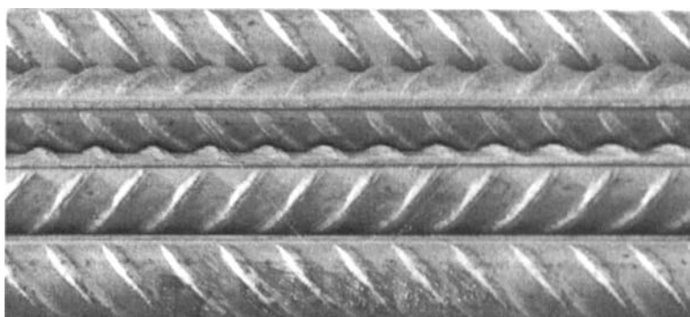
Fig. 13.6 High yield strength deformed bars
