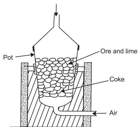
Fig. 14.5 Roasting of Lead Ore in Sinterer
