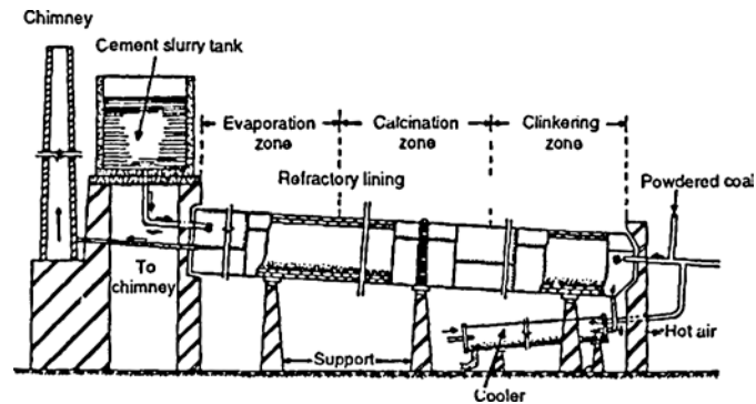
Fig. 5.3 Rotary Kiln
