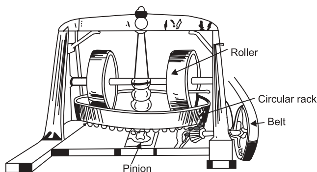
Fig. 12.4 Power Driven Mortar Mill (Pan Mill)
