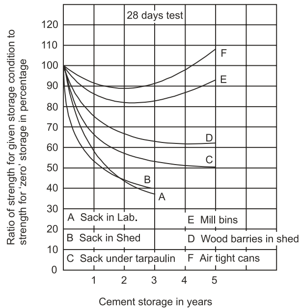
Fig. 10.24 Effect of Storage of Cement on Strength of Concrete
