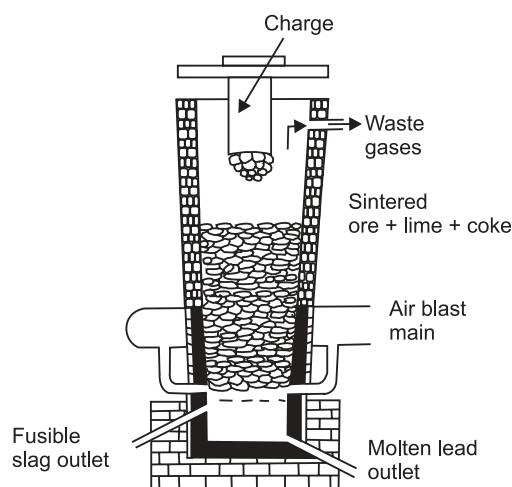
Fig. 14.6 Smelting of Galena in Blast Furnace
