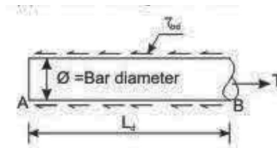
Figure 1.13 Development length of bar
