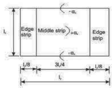
Figure 2.3 (a): For Span l_x
