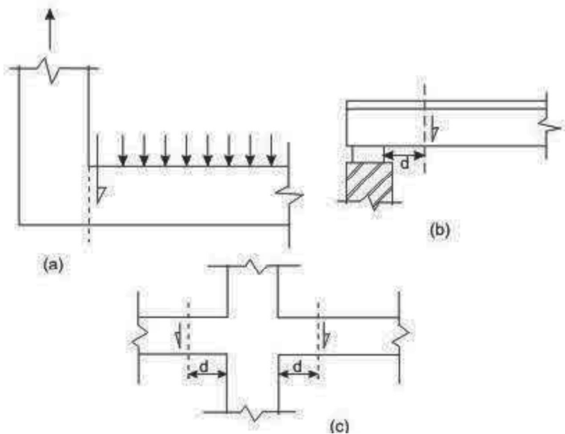
Figure 1.12 Support condition for locating factored shear force
