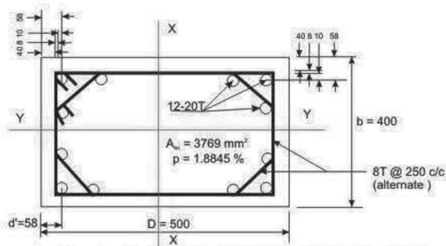
Reinforcement Detailing
