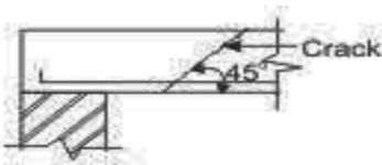
Figure 1.10 (a) Web shear progress along dotted lines
