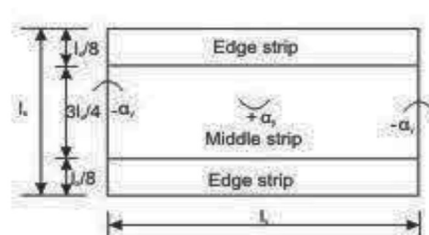
Figure 2.3 (b): For Span l_y
