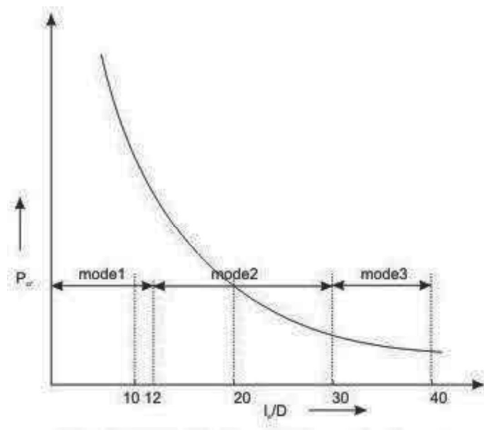
Figure 3.3 Modes of failure of columns
